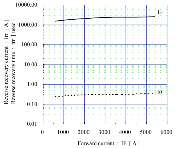
Reverse recovery characteristics (typ.) Vcc=600V, VGE=±15V, Rgon=0.5Ω, Tj=125°C
