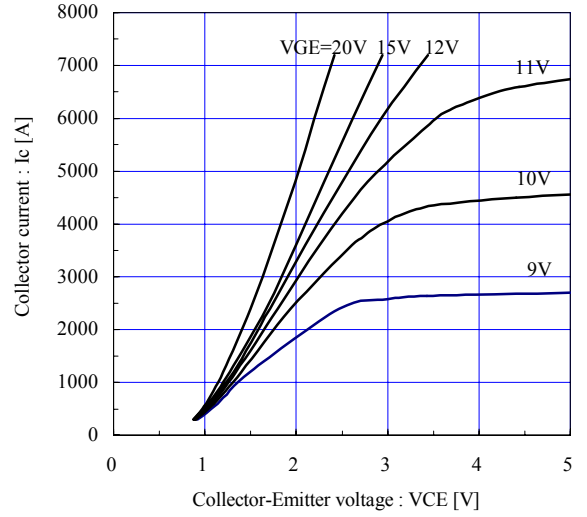
Collector current vs. Collector-Emittter voltage (typ.) Tj= 125°C, sense terminal
